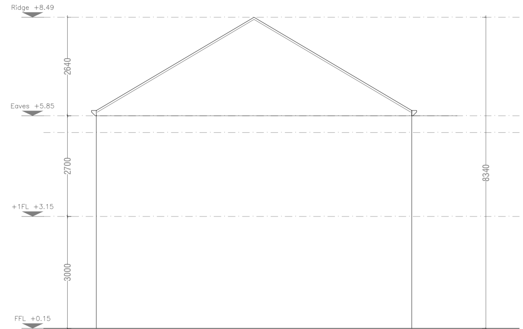
House Type T1 Semi-Detached Side Elevation
