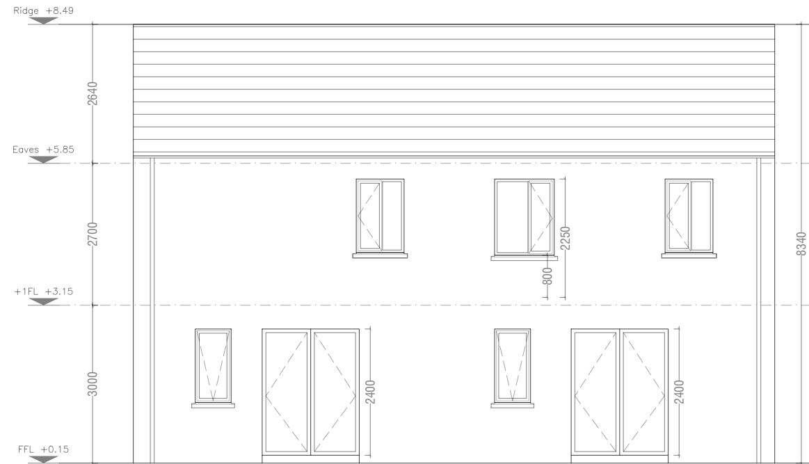
House Type T1/ T2 Semi-Detached Rear Elevation
